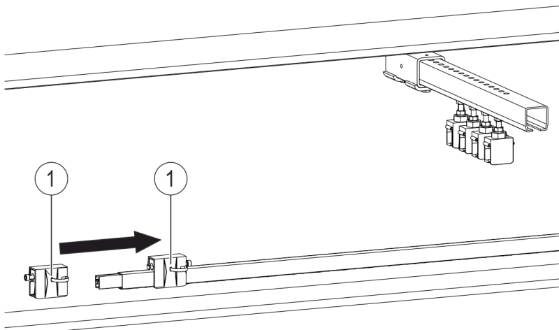
Fig. 91: Slide the anchor point clamps 0812 onto the conductor rail
