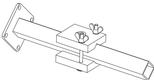
Fig. 42: Drilling jig
