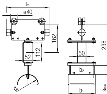
Towing Trolley
