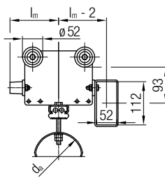
Towing Trolley
