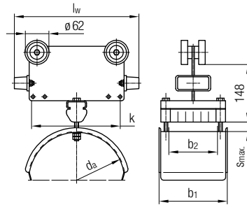
Cable Trolley
