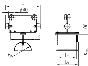
Cable Trolley
