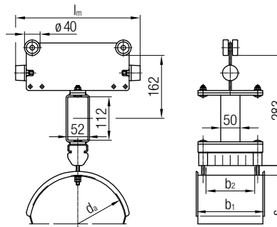
Towing Trolley
