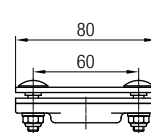
End Clamp
