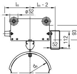
Towing Trolley
