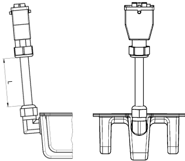
90° connection
