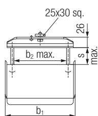
End Clamp
