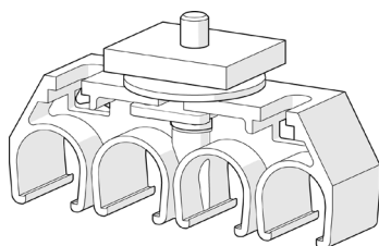
Fig. 9: Hanger clamp 0811 (with fastening components for C-rail)
