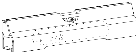
Fig. 34: Two-piece connector cap with bayonet connector
