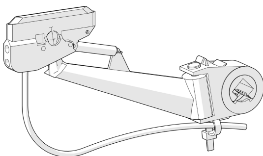
Fig. 30: Current collector 081102, long-arm version, 63 mm
