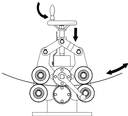
Fig. 27: Bending device (081081)
