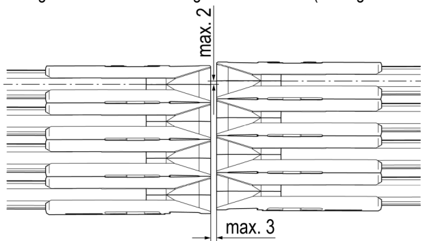
Fig. 59: Maximum deviation horizontal
