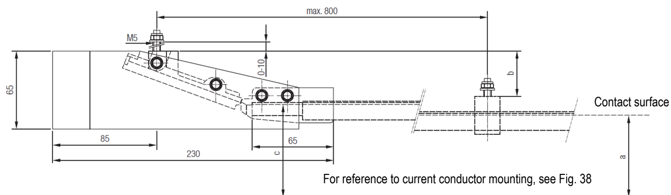
Fig. 93: Pickup guide 081182 – short version
