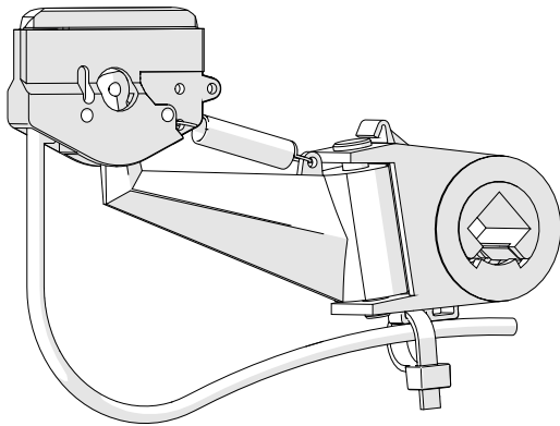
Fig. 16: Single current collector, short-arm version, 40 mm
