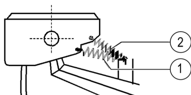
Fig. 63: Stabilizing spring for towing and reversing operation
