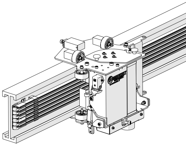
Fig. 19: Rail cleaner
