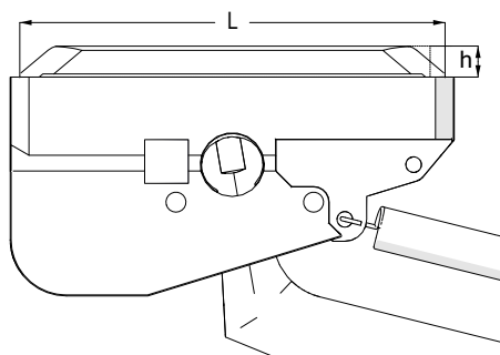
Fig. 2: Sliding contact length and wear height
