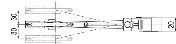
Fig. 57: Long-arm current conductor with long sliding contact (63 mm)
