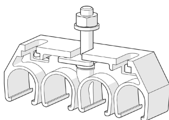
Fig. 8: Hanger clamp 0811 (screw-on, e.g. on mounting bracket)
