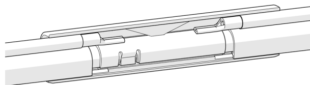
Fig. 20: Infeed connector with crimp connection 100 A and PE/Protective conductor connection, max. 10 mm 2
