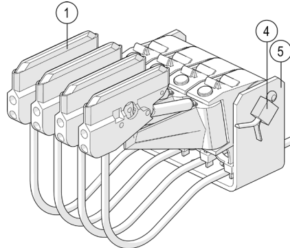
Fig. 62: Mounting of the current collector with the support bracket
