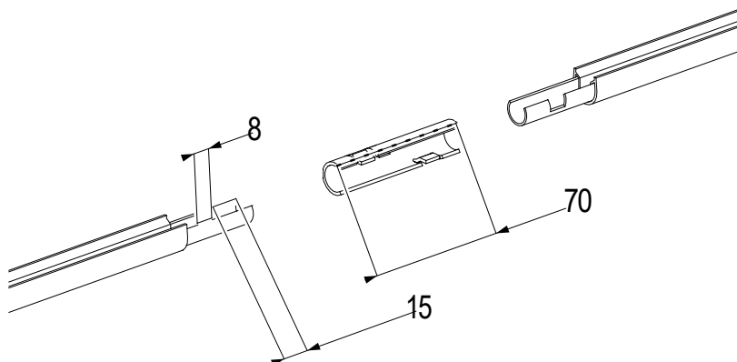
Fig. 61: Dimensions of the bayonet connector, tab and notch
