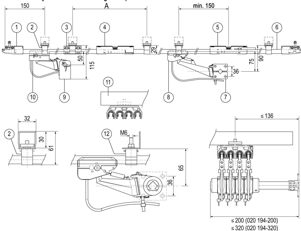
Fig. 42: Components in a conductor rail system
