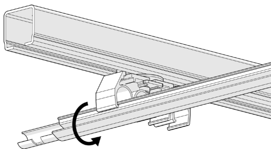
Fig. 30: Screw rail into hanger clamp
