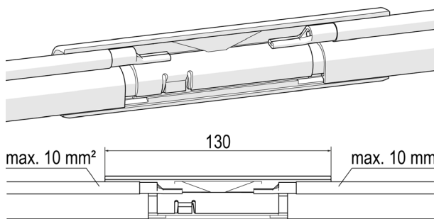
Fig. 47: Electrical feed with connector 100 A
