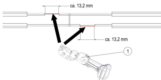
Fig. 9: Make a notch for expansion units with a notching and cutting tool (1)
