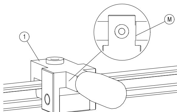
Fig. 41: Lay the drilling jig on the marking
