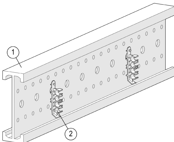
Fig. 28: Clip-on hanger clamps on EMS profile with existing holes (example)
