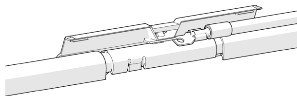
Fig. 10: Infeed connector with flat plug connection 35 A (not for PE/Protective conductor connection), 4-6 mm 2
