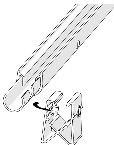
Fig. 70: Turn anchor point
