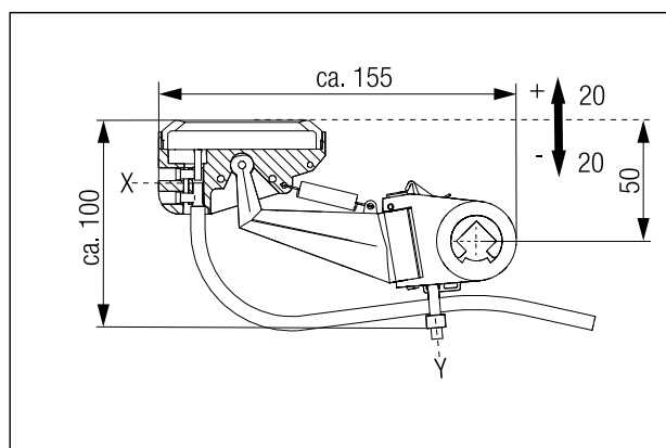
Fig. 55: Short-arm current collector with short sliding contact (40 mm)
