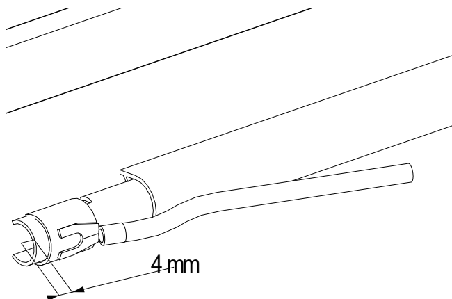
Fig. 49: Distance from conductor bar to feed shoe
