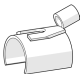
Fig. 13: Feed shoe with crimp connection
