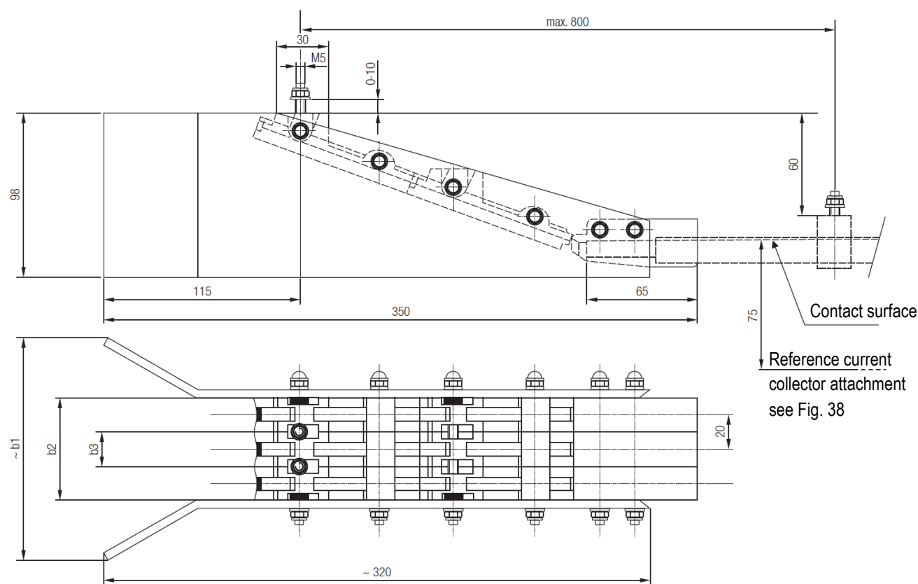
Fig.54: Pickup guide 081182 - long version
