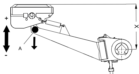
Fig. 3: 081101 and 081102 installation clearance and contact force
