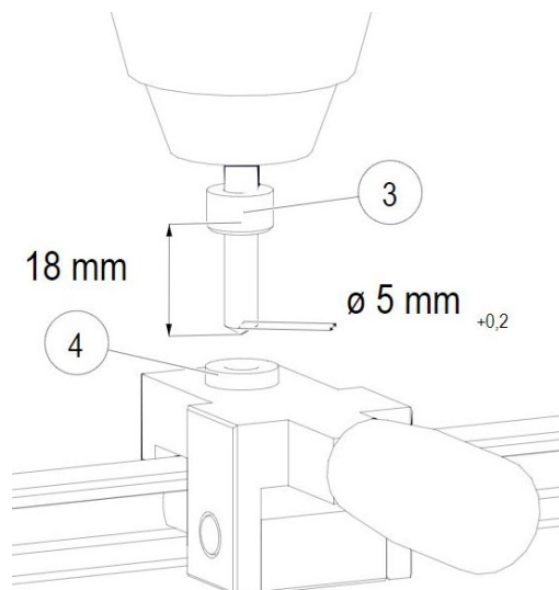
Fig. 42: Hole for anchor point drilled
