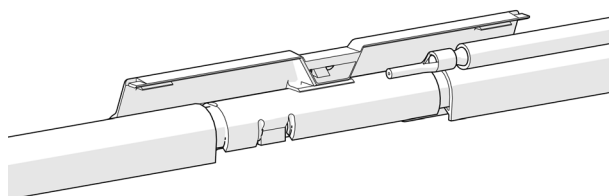
Fig. 11: Infeed connector with crimp connection 45 A and PE/Protective conductor connection, 4-6 mm 2
