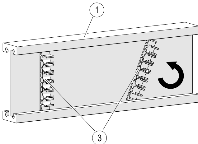
Fig. 29: Clip-on / Screw-in hanger clamp on EMS profile without existing holes (example)
