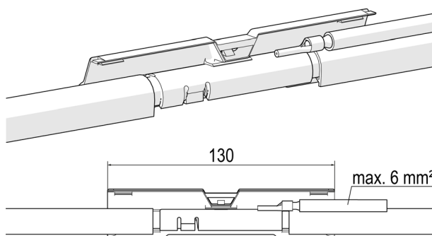
Fig. 83: Electrical feed with connector 45 A
