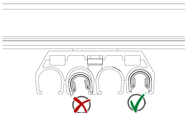
Fig. 32: Comparison of correctly and incorrectly engaged rail
