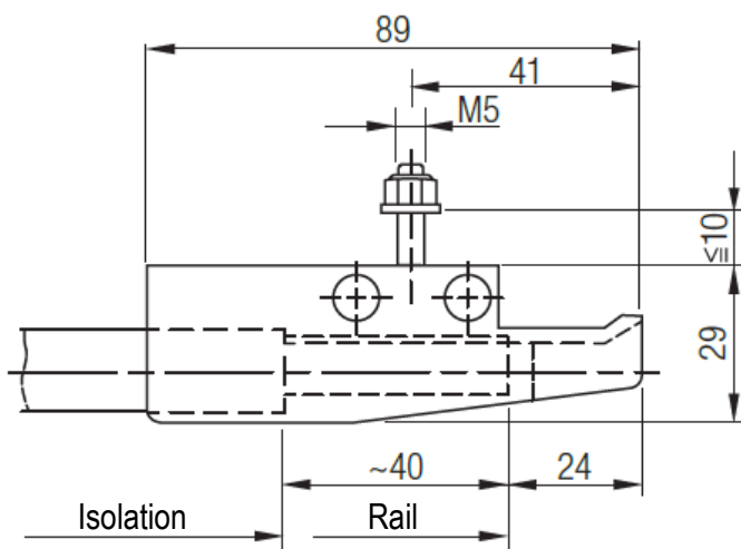
Fig. 80: Dimensional drawing: End cap 081174 Insulation profile - Conductor bar
