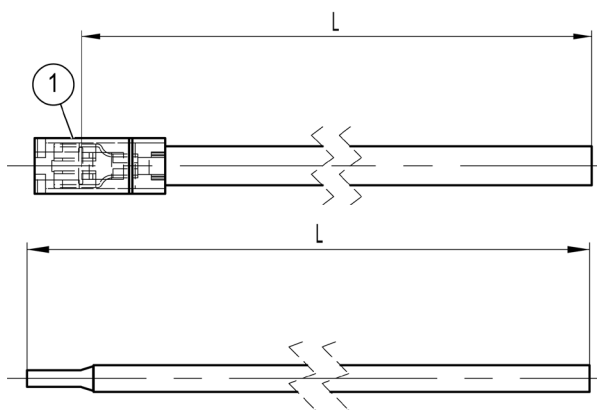
Fig. 33: Connection cable for current collector 081101/02
