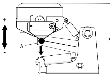
Fig. 4: 081106 installation clearance and contact force
