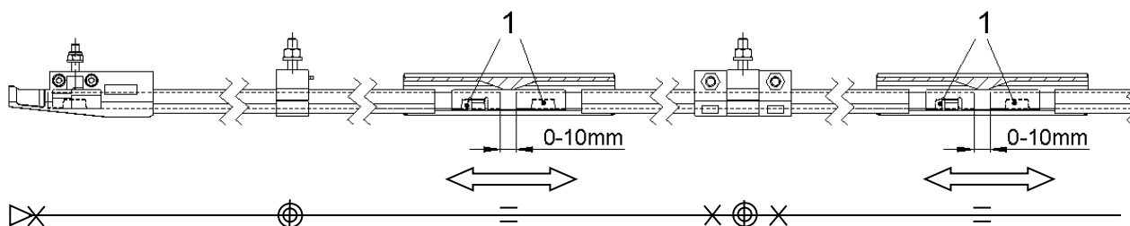
Fig. 38: Schematic view: Function of the expansion points in the expansion unit
