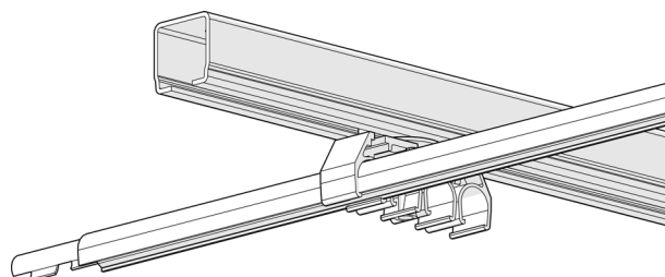
Fig. 31: Rail screwed into hanger clamp
