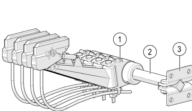
Fig. 61: Mounting the current collector on the outrigger
