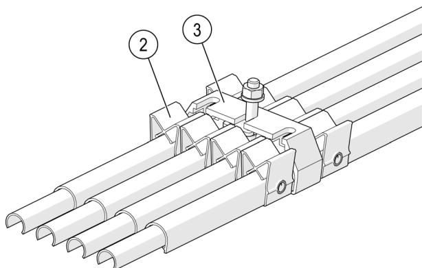
Fig. 12: Anchor point
