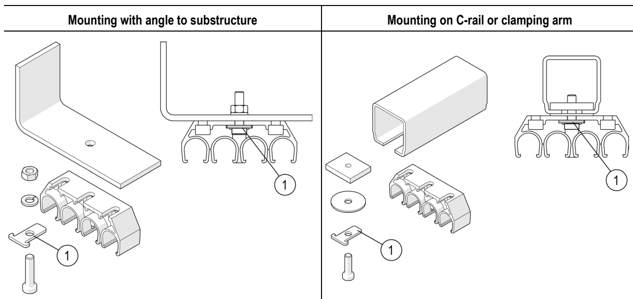
Fig. 51: Screw-on hanger clamps with insert (1)
