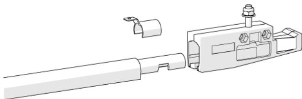
Fig. 21 End cap for rail ends and transfers
