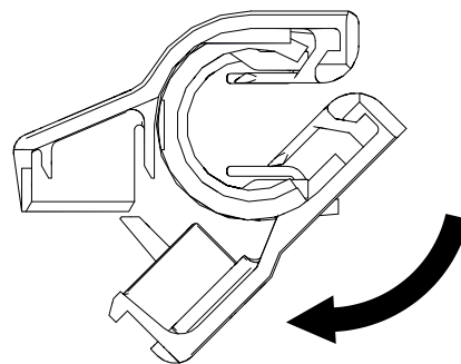
Fig. 36: Clip the second cap half onto the rail
