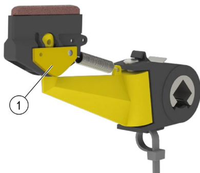
Fig. 64: Current collector with lateral spacers
