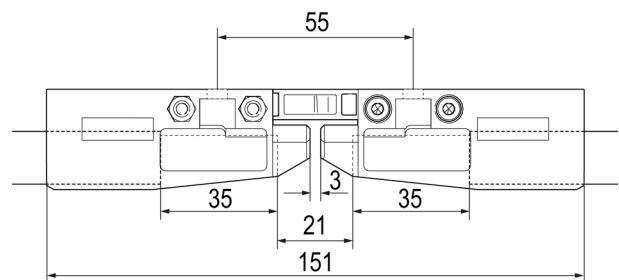
Fig. 45: Mounting dimensions of the air gap
