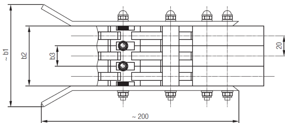
Fig. 53: Pickup guide 081182 – short version
