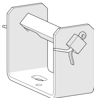
Fig. 32: Support bracket for single current collector
