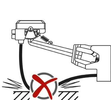
Fig. 100: Connection cable must not abut
