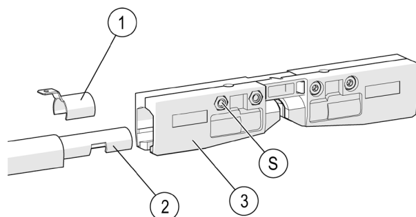
Fig. 51: Infeed at the air gap
