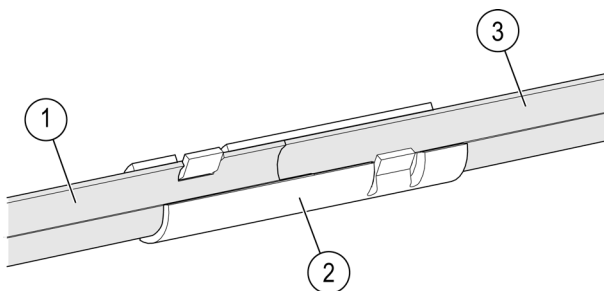
Fig. 8: Rail connector (illustration turned, view without connector cap)
