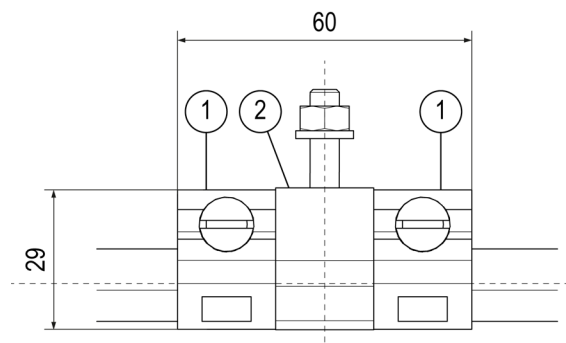
Fig. 43: Mount anchor points
