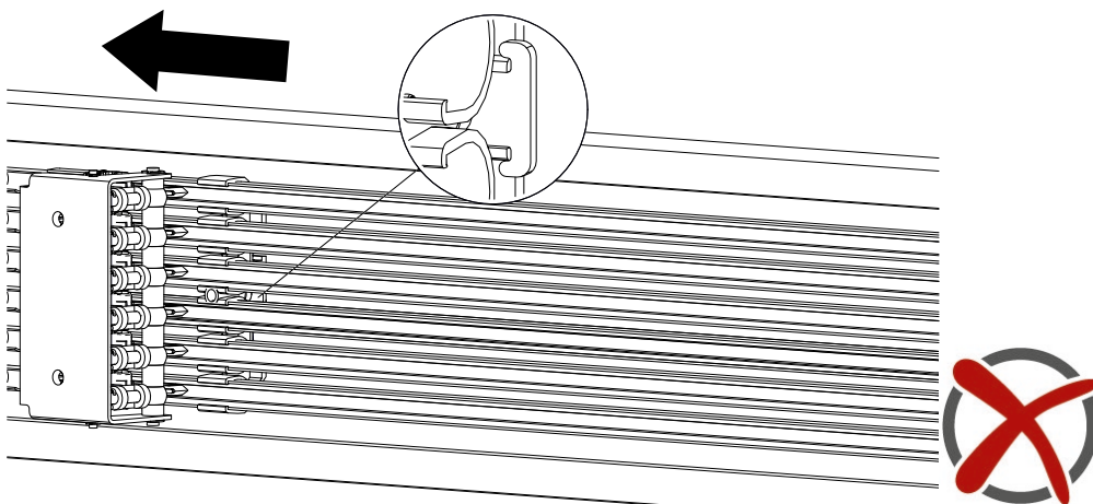
Fig. 53: Insert is mounted against the travel direction of the current collector
