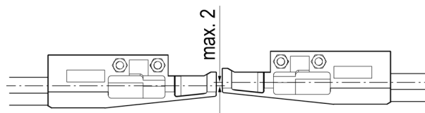
Fig. 60: Maximum deviation vertical
