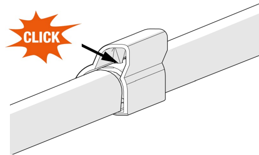
Fig. 63: Engage one-piece connector cap
