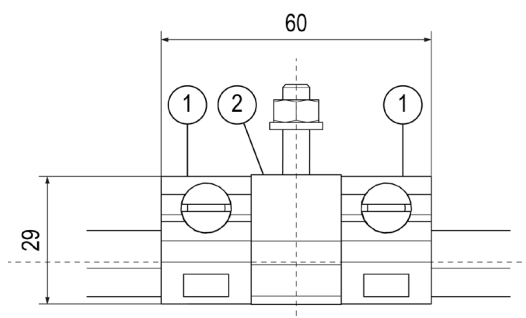
Fig. 13: Anchor point (securely seated)
