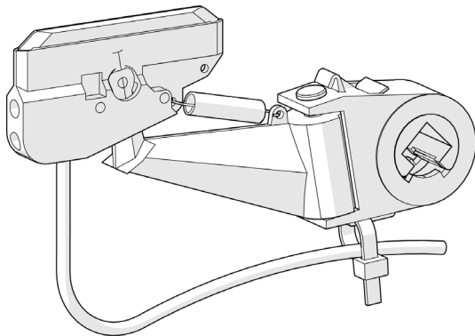
Fig. 17: Current collector 081101, short-arm version, 63 mm
