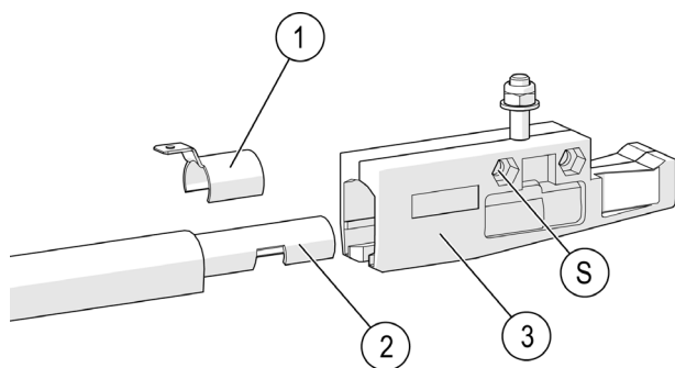
Fig. 50: Infeed on the end cap
