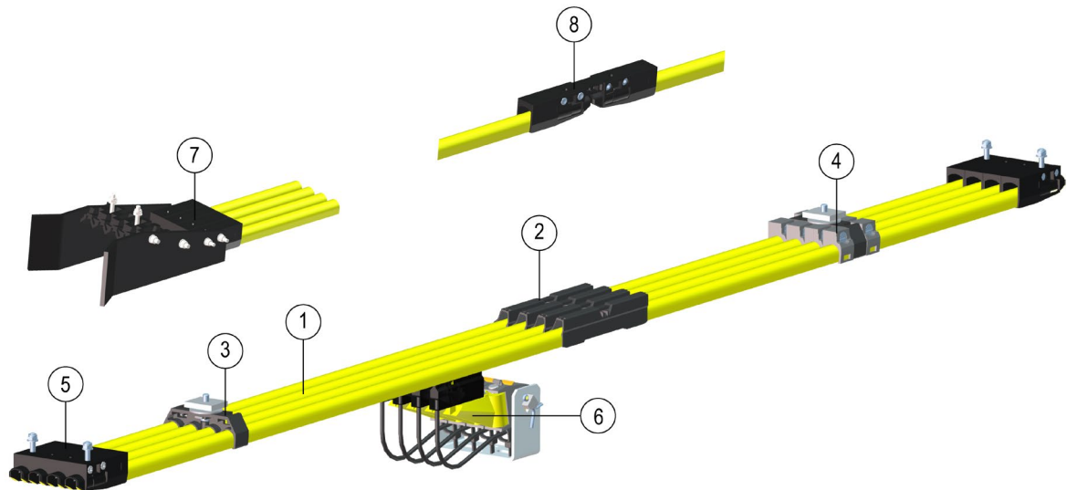
Fig. 6: System overview
