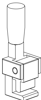
Fig. 40: Drilling jig for PH/PE rails
