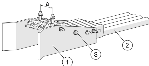
Fig. 52: Pickup guide short version
