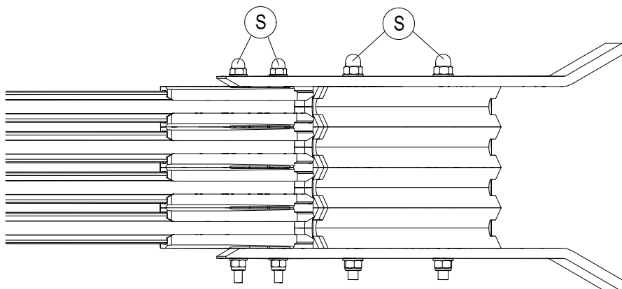
Fig. 91: Slightly loosen the four side screws (S)
