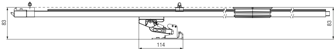
081507 – Single Current Collector
