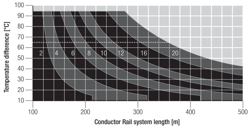
Diagram 3 – Number of Connector/Expansion Units when using Copper Rails > 100 m
