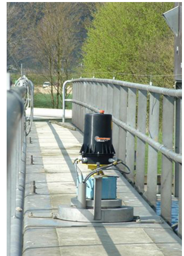
Slip ring assembly in circular scraper (sewage treatment plant)
