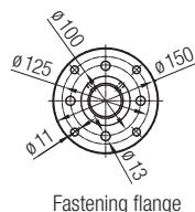
Fastening flange
