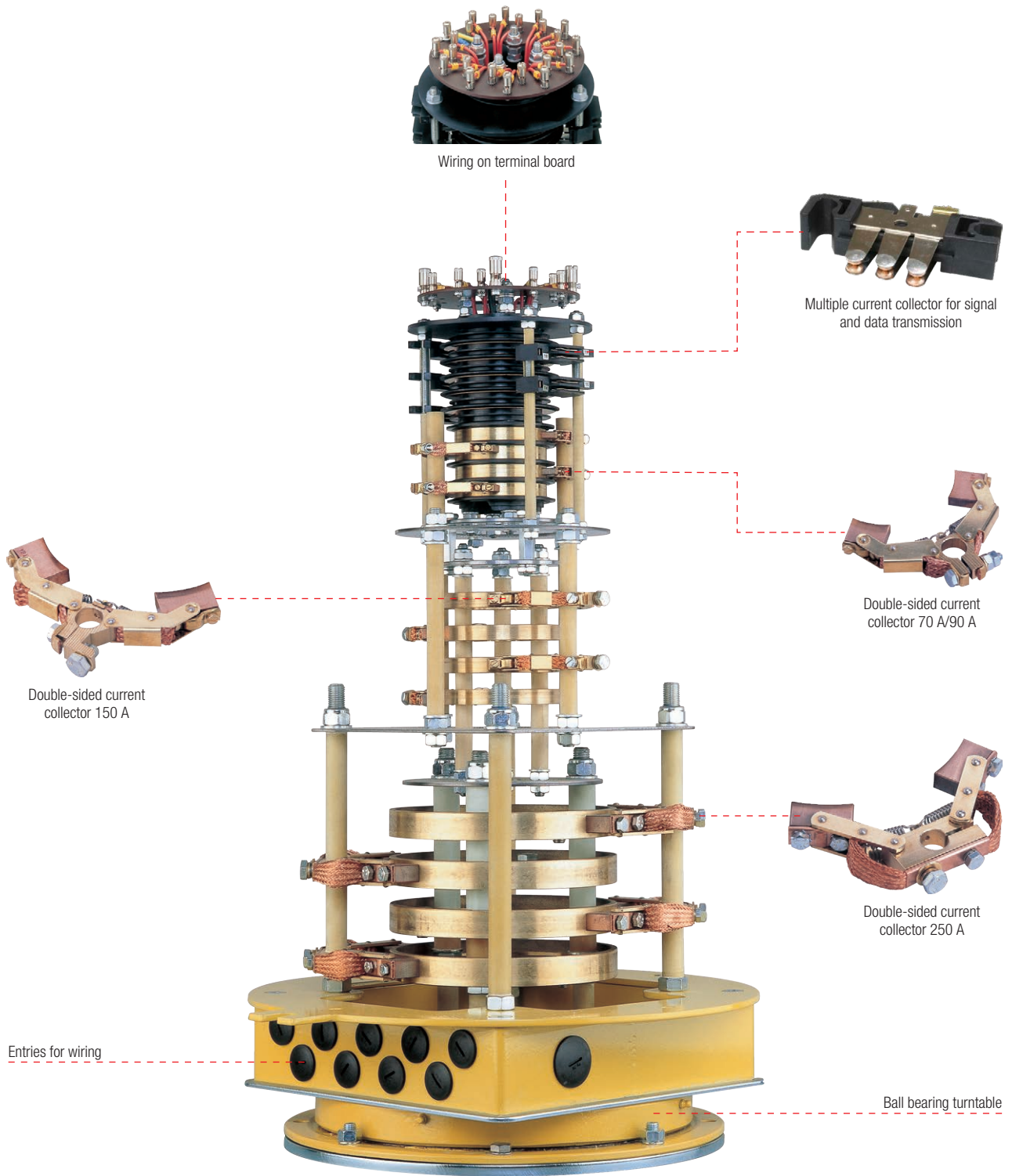
Combined Slip Ring Assembly GS2104 / 1904 / 1504 / 1806 / 04 ML 3x250 A + PE + 4x150 A + 4x70 A/90 A + 6x21 A + 4x data
