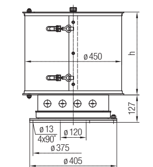
With ball bearing turntable and split cover
