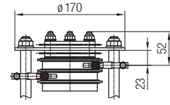
Version with support disk for 8 rings
