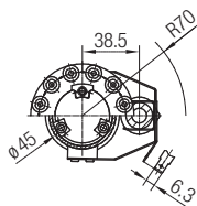
12 poles with sheath clamps
