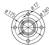
Fastening flange
