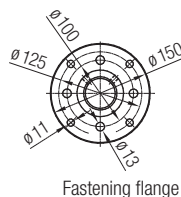
Fastening flange
