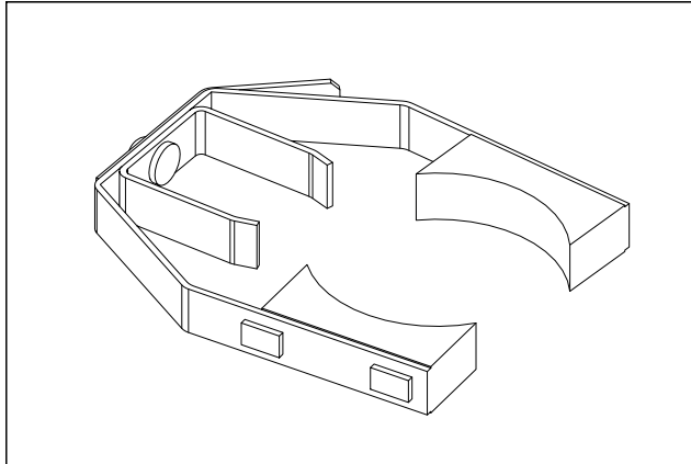
Fig. 2: Current collector
