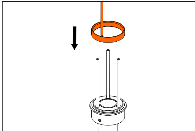
Fig. 24: Mount new PE+ slip ring with strand.
