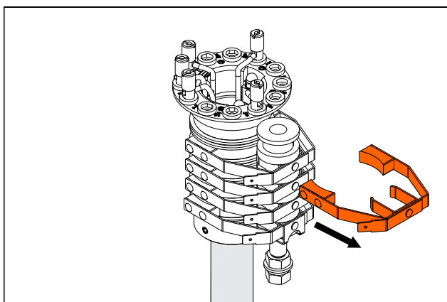
Fig. 12: Pull PH+ current collector from the insulator. Disassemble all PH+ current collectors in the same way.
