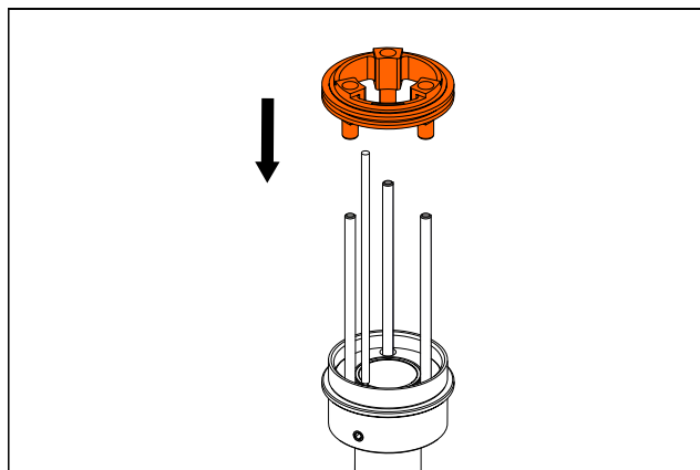
Fig. 25: Place insulating body onto the slip ring studs. Install all slip rings and insulating bodies in the same way.
