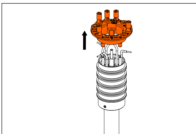
Fig. 21: Remove terminal block.
