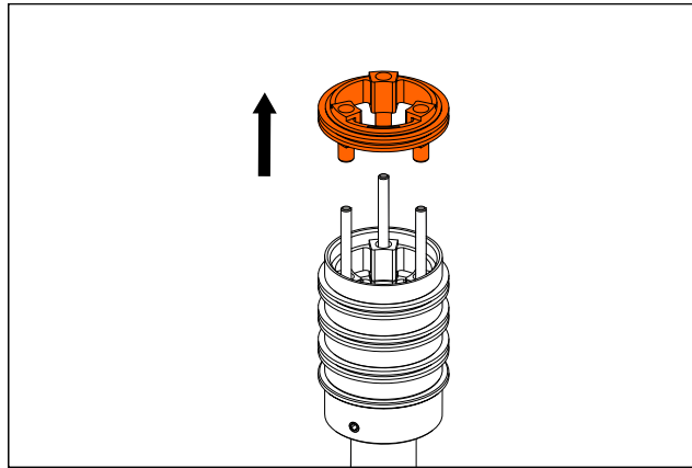
Fig. 23: Remove insulator.
