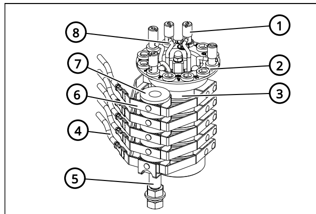
Fig. 1: Type 45/1 Build-in slip ring assembly
