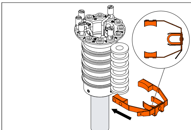
Fig. 15: Mount new PE+ current collector with bracket over the insulator onto the PE+ slip ring. Check the alignment of the current collector with the slip ring.
