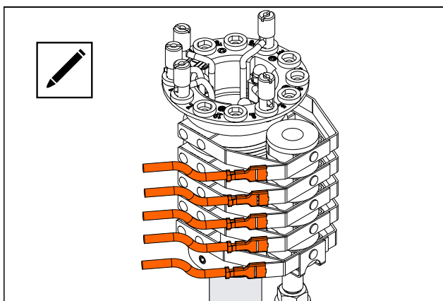
Fig. 10: Label connecting cables.
