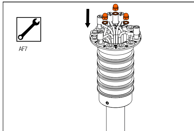
Fig. 27: Tighten inner cap nuts on the terminal block.
