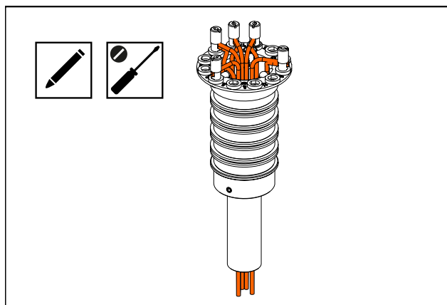
Fig. 19: Label the connecting cables and disconnect the connecting cable ends from the mantle terminals.
