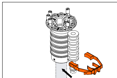
Fig. 7: PE+ current collector onto the insulator.
