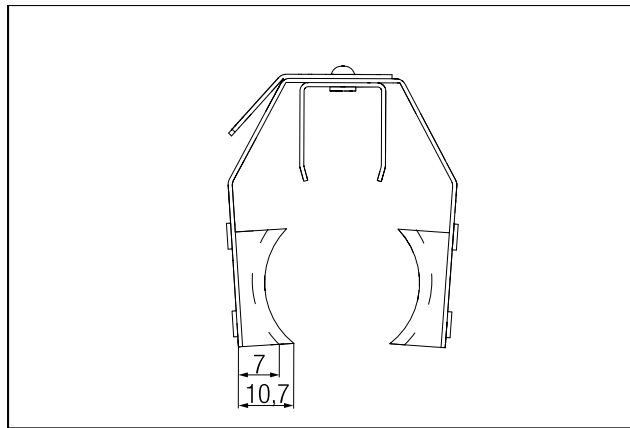
Fig. 9: Sliding contact wear limits for Types 45/1, 45/2 and 45/3
