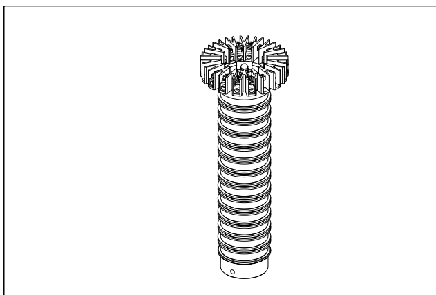
Fig. 5: Ring assembly with vertical terminal block for Type 45/1
