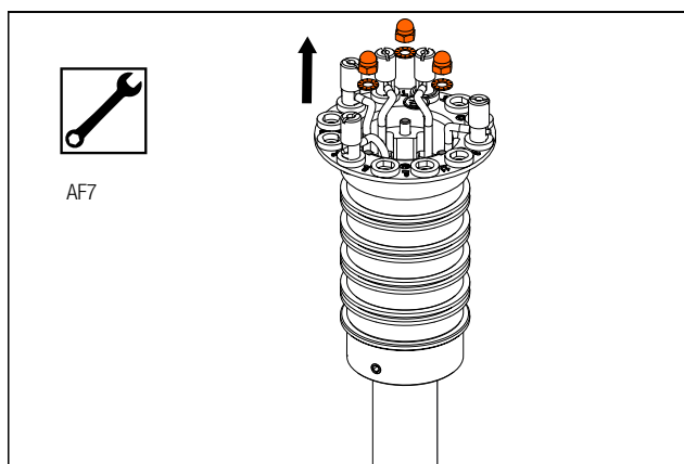
Fig. 20: Loosen inner cap nuts from the terminal block.
