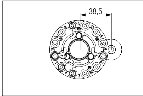
Fig. 8: Distance from insulator to slip ring diameter
