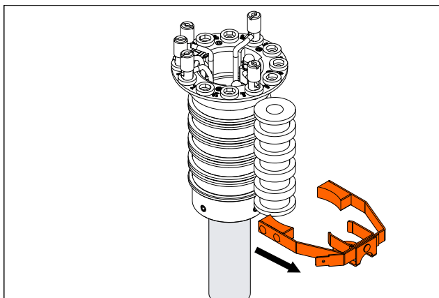
Fig. 14: Remove the PE+ current collector from the insulator.
