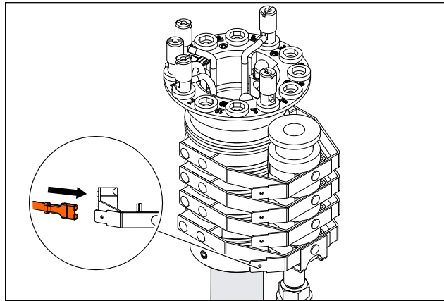
Fig. 18: Connect current collector connecting cables according to the connection diagram. Check that the flat plug is securely attached to the current collector. If necessary, bend or replace the flat plug.
