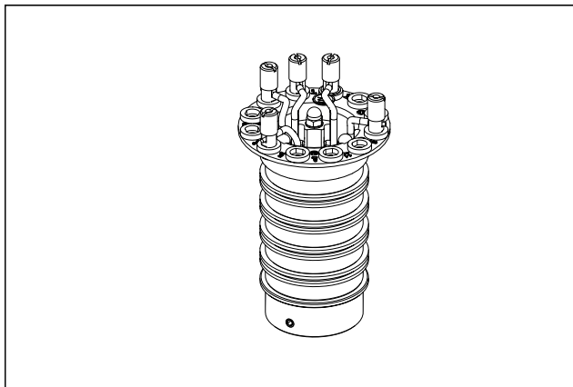
Fig. 4: Ring assembly with standard terminal block
