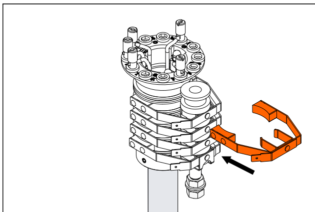
Fig. 17: Mount PH+ current collector over the insulator onto the PH+ slip ring. Mount all PH+ current collectors in the same way.
