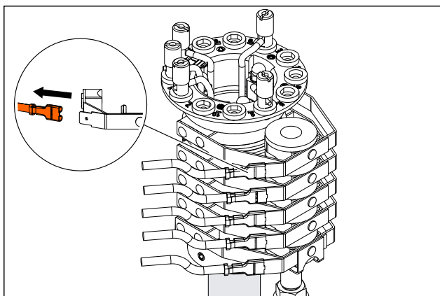
Fig. 11: Disconnect connecting cables from the current collector.
