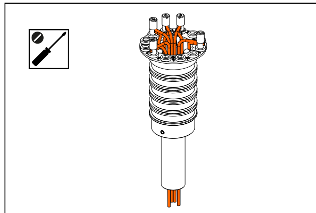
Fig. 28: Trim new cables to correct length for the terminals and strip the cable ends. Secure connecting cable ends in the mantle terminals according to the terminal connection table.
