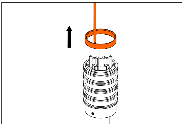
Fig. 22: Remove slip ring with strand.
