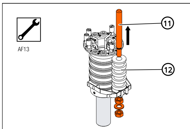
Fig. 13: Loosen the brush bolt to remove the PE+ current collector from the insulator.
