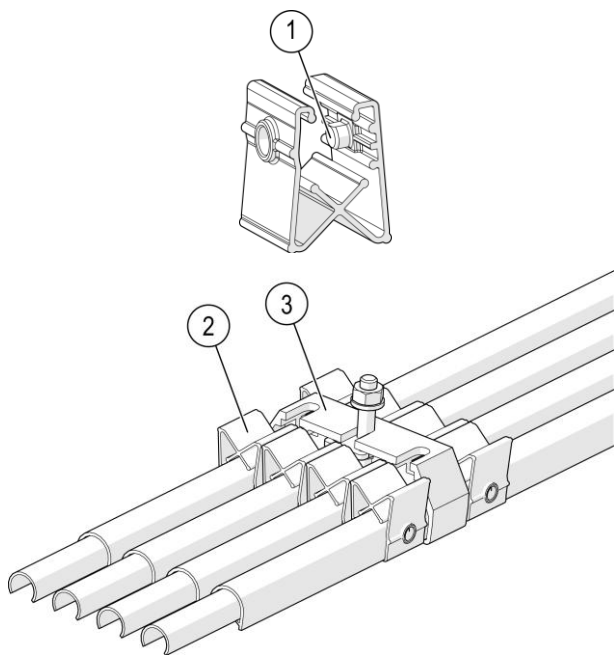
Fig. 8: Anchor point
