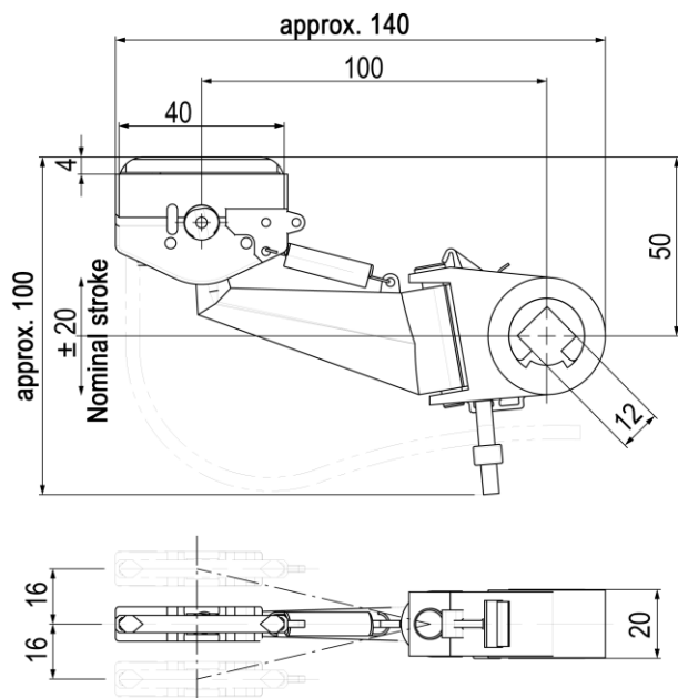
Fig. 92: Short-circuit current collector with short sliding contact (40 mm)
