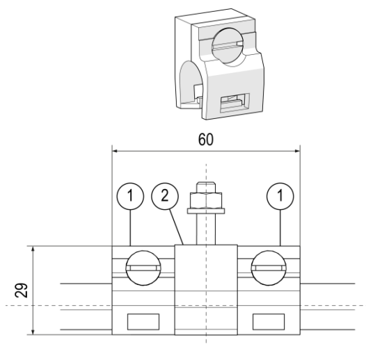
Fig. 9: Anchor point (securely seated)
