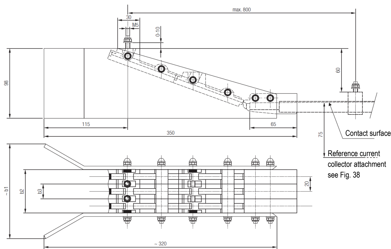
Fig.91: Pickup guide 081182 - long version
