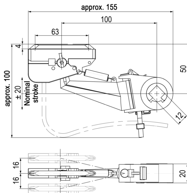
Fig. 93: Short-circuit current conductor with long sliding contact (63 mm)
