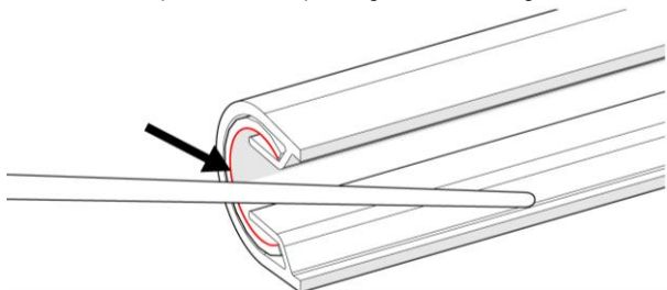
Fig. 40: Deburr the conductor rail with a smooth file
