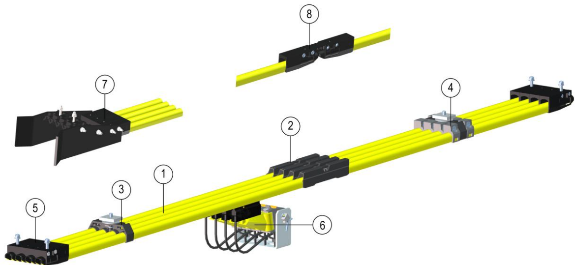
Fig. 2: System overview
