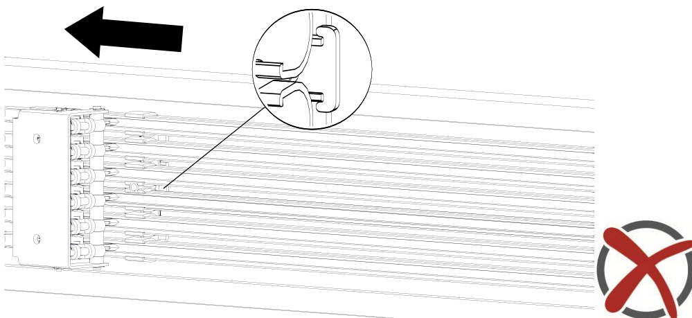
Fig. 49: Insert is mounted against the travel direction of the current collector
