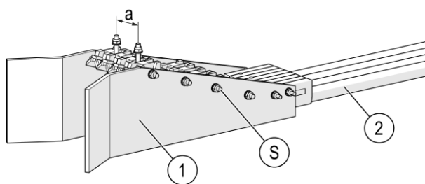
Fig. 86: Pickup guide long version
