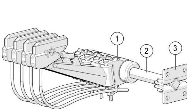
Fig. 102: Mounting the current collector on the outrigger
