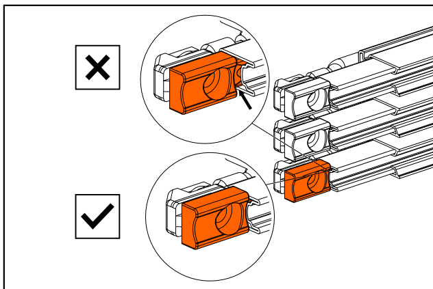
Fig. 27: Correct position of power feed terminal on conductor bar
