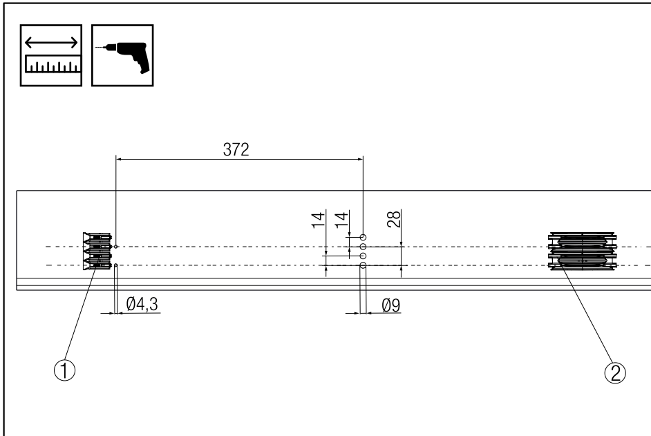
Fig. 13: Spacing in a combined system: 2-pole and 2-pole
