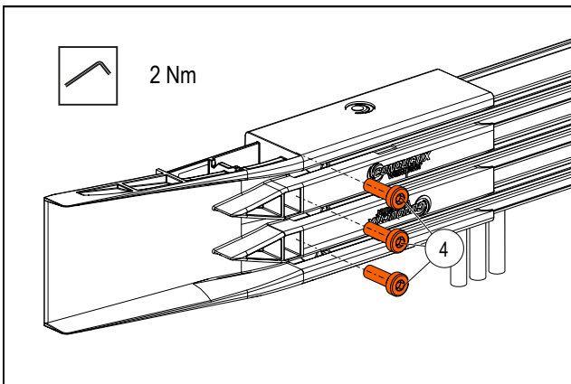
Fig. 29: Tighten cylinder screws (Pos. 4)
