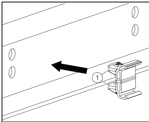
Fig. 19: Insert hanger clamp (Pos. 1) clips into hole
