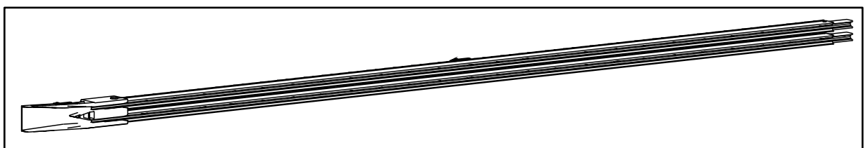
Fig. 3: Conductor rail with pickup guide (single-sided)
