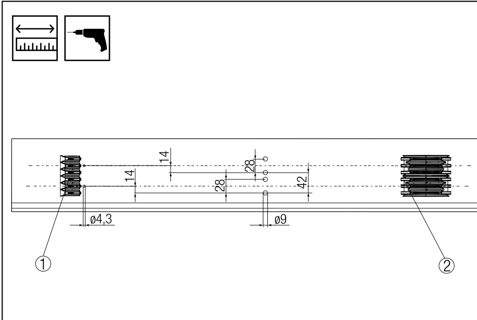
Fig. 14: Spacing in a combined system: 3-pole and 3-pole
