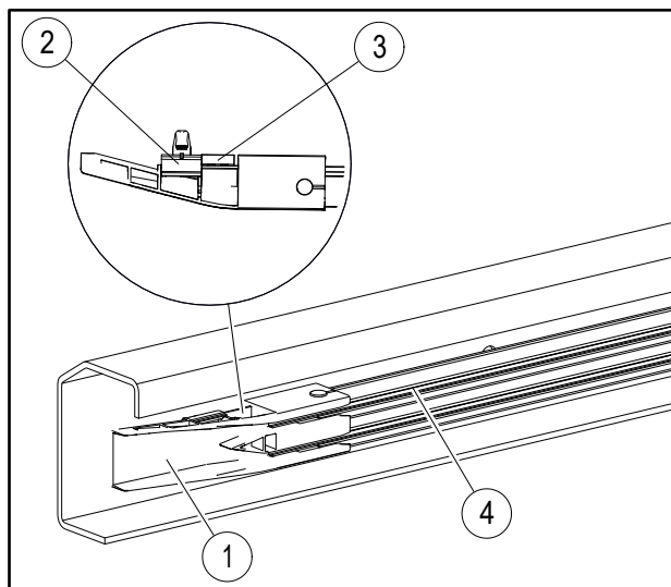
Fig. 33: Conductor rail (Pos. 4) cannot expand
