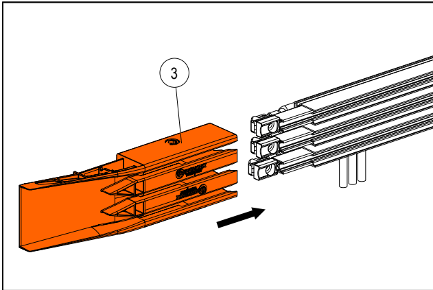
Fig. 28: Slide guide (Pos. 3) over conductor rail end
