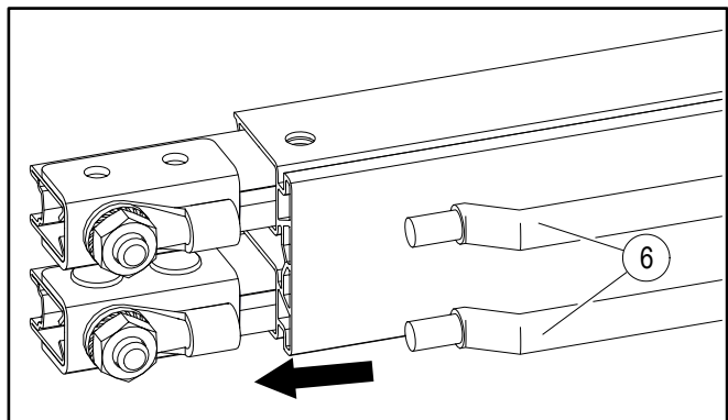
Fig. 23: Crimp connection cables with crimping cable lug
