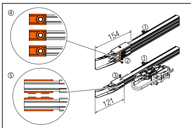
Fig. 10: Differences and similarities between pickup guide
