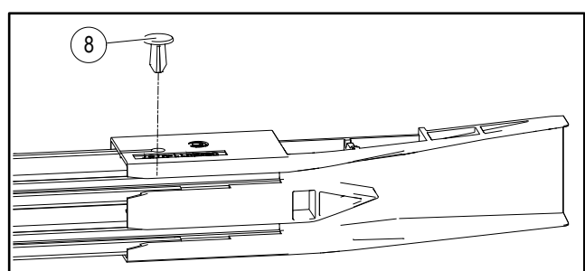
Fig. 25: Tap expanding rivet into hole
