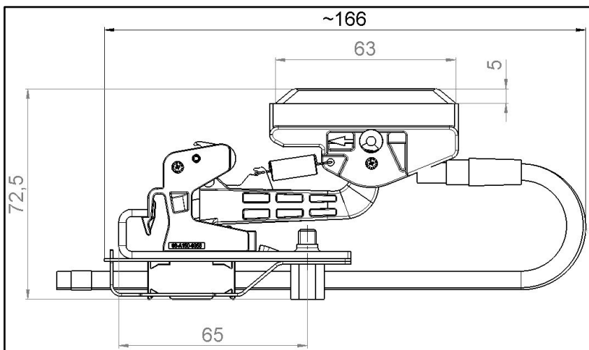
Fig. 41: Current collector installation dimensions
