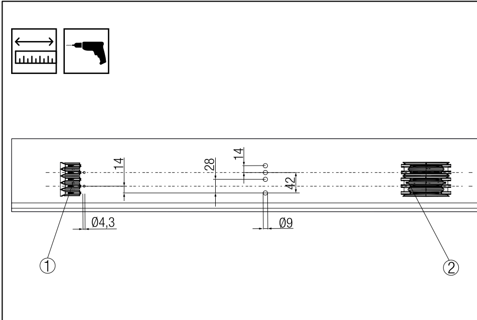
Fig. 15: Spacing in a combined system: 2-pole above and 3-pole below
