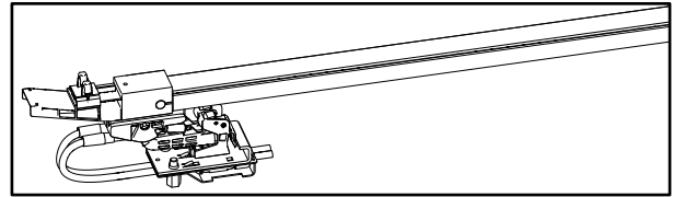
Fig. 43: Current collector inserted from below
