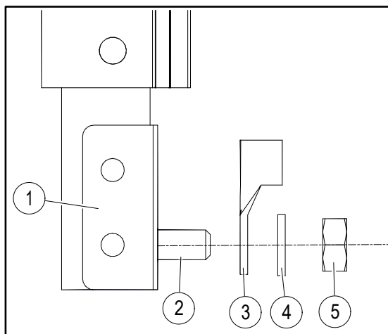
Fig. 22: Screw on crimping cable lug
