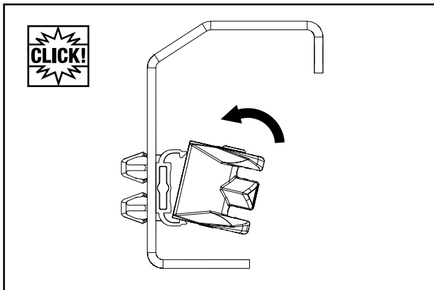
Fig. 40: Hook rail into hanger clamp
