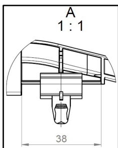
Fig. 37: Sliding bearing
