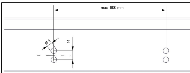
Fig. 12: Drilling pattern for 2-pole hanger clamp spacing
