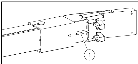
Fig. 4: Anchor point 0865/sliding bearing
