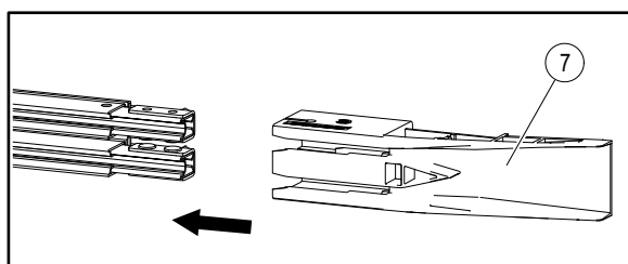
Fig. 24: Slide pickup guide over power feed point
