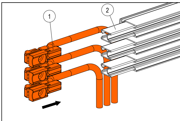
Fig. 26: Slide power feed terminals (Pos. 1) into the conductor bar (Pos. 2) Slide the terminal into the PE conductor bar.
