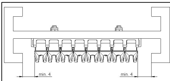
Fig. 11: Side clearance min. of 4 mm (Illustration does not correspond to the product described here)
