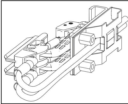
Fig. 7: Current Collector 0865
