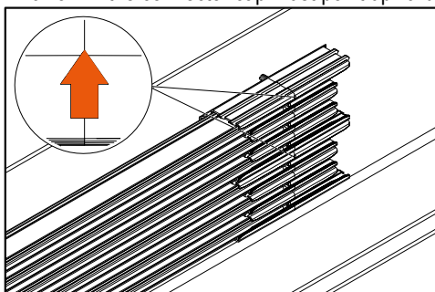
Fig. 39: Observe connector cap orientation
