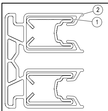
Fig. 6: Conductor Rail 0865
