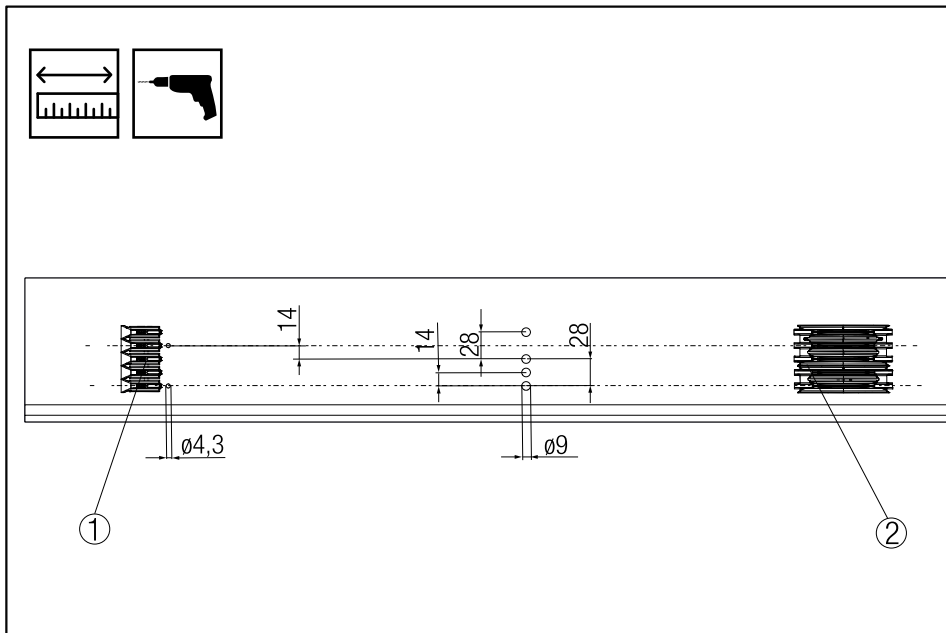
Fig. 16: Spacing in a combined system: 3-pole above and 2-pole below
