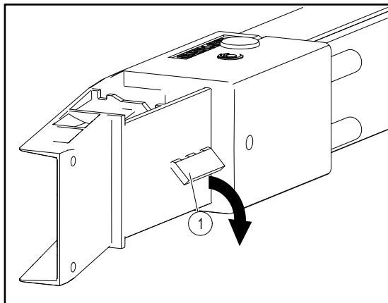
Fig. 34: Break away fixing web (Pos. 1)
