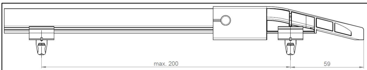
Fig. 17: Pickup guide without fixing web
