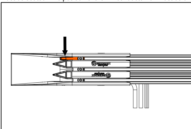
Fig. 30: PE terminal seated in guide recess
