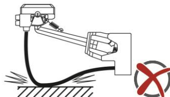
Fig. 32: Connection cable must not rest
