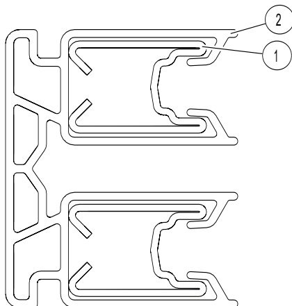
Fig. 8: Conductor Rail 0865
