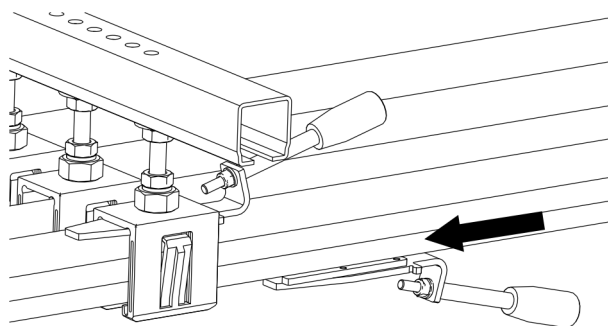
Fig. 65: Insert Tool 2 on the open side of the conductor rail
