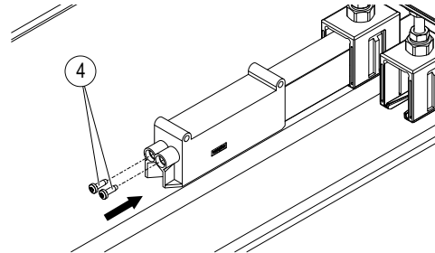
Fig. 102: Tighten raised countersunk screws
