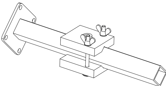
Fig. 38: Drilling jig
