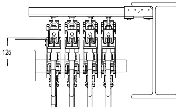
Fig. 110: Nominal mounting dimension 125 mm
